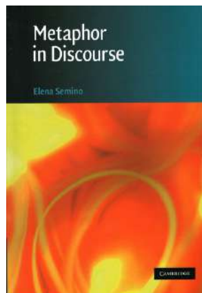
Semino, Elena. Metaphor in discourse. Cambridge, UK : Cambridge University Press
